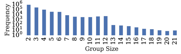
Figure 3: Group size check-in frequency (logarithmic scale).
