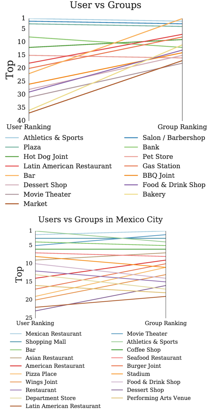
Figure 6: Category comparison using the check-ins of a single user and her groups. The Kendall-tau is 0.1(top). Total check-ins count for all the users and groups in Mexico City. The Kendall-tau is 0.8(bottom).
