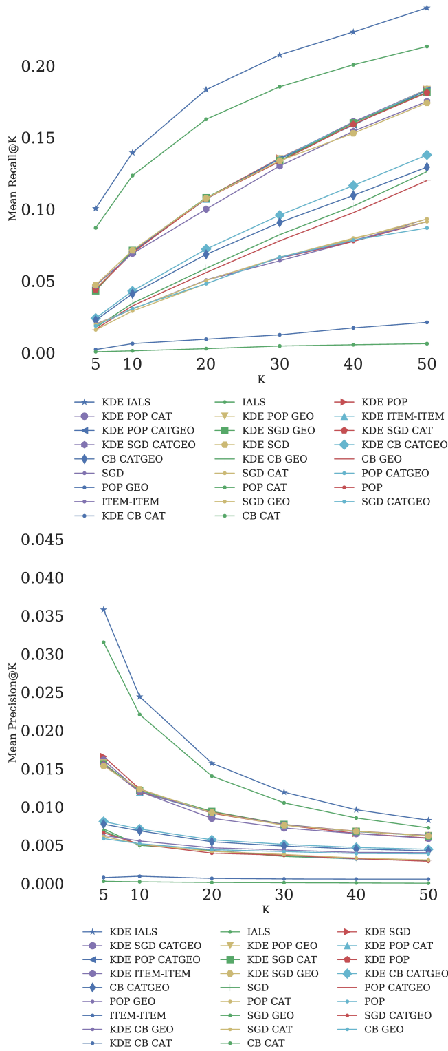
Figure 11: Istanbul Recall@K(top) and Precision@K(bottom). The legends are sorted by the best performance models from left to right and top to bottom.
