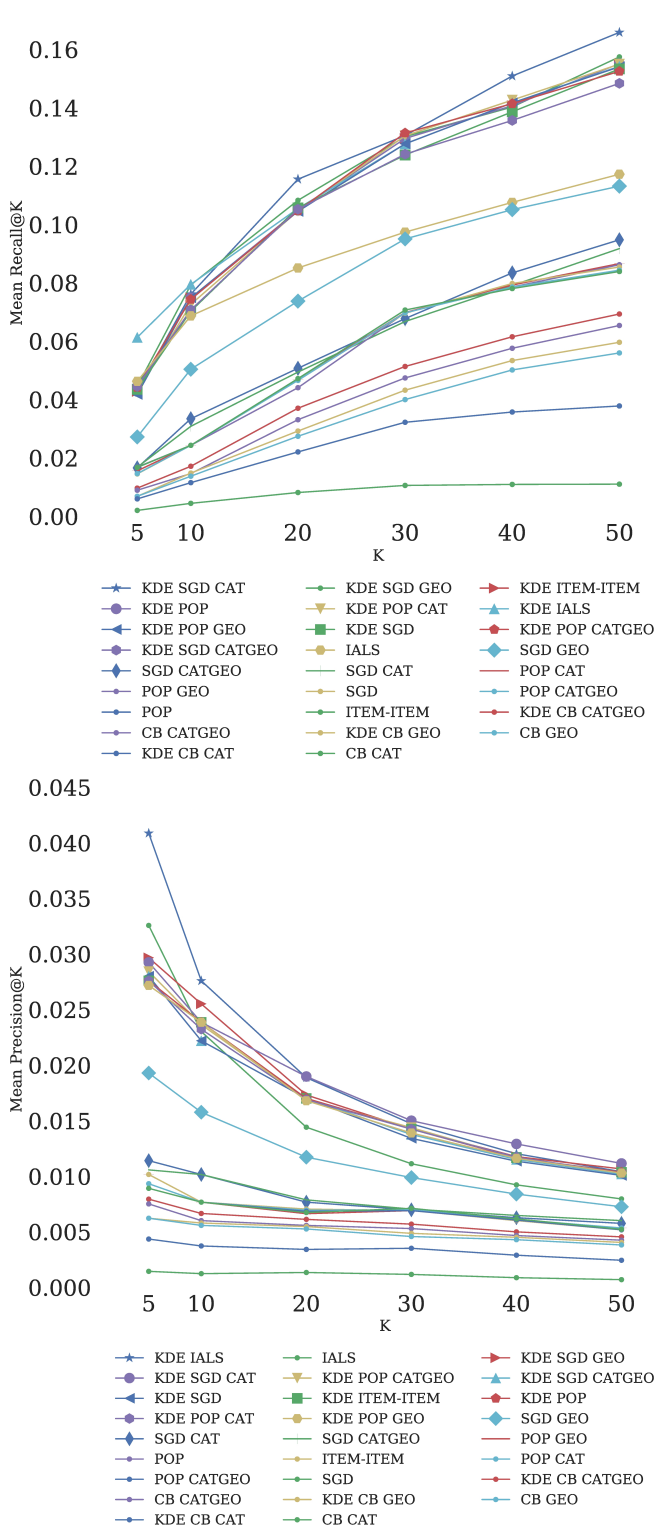
Figure 13: Mexico City Recall@K(top) and Precision@K(bottom). The legends are sorted by the best performance models from left to right and top to bottom.
