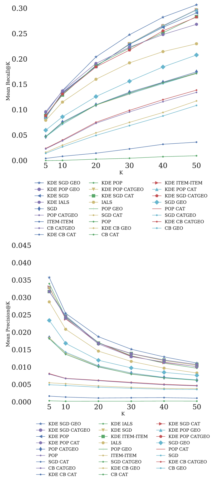
Figure 12: Izmir Recall@K(top) and Precision@K(bottom). The legends are sorted by the best performance models from left to right and top to bottom.
